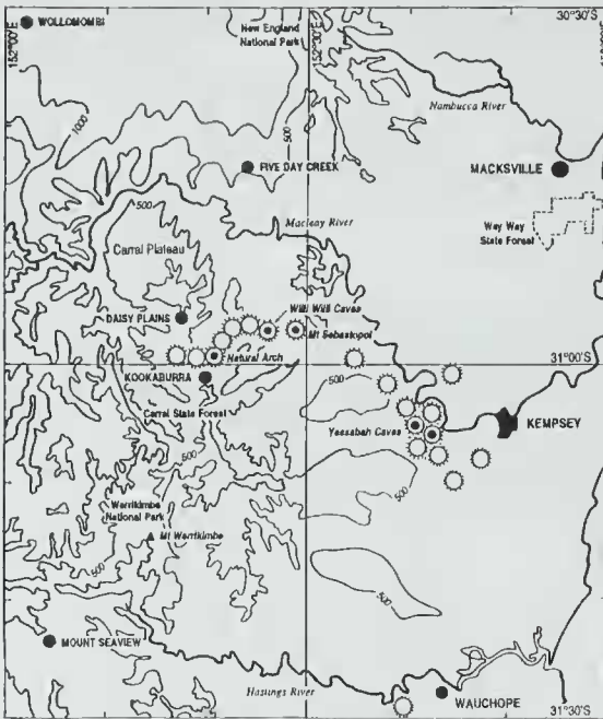
Figure 1. Study area. Limestone outcrops represented by spiked circles.
